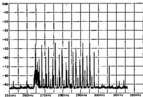
Figure 1. Baseband recording using the 3595A.
