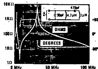
Fig. 1 Wide impedance excursions are displayed in log form, along with the phase angle. Here, a series-parallel resonant circuit is characterized for resonances and anti-resonances up to 100 MHz.
