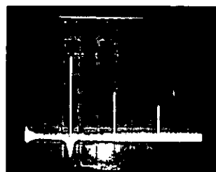
FIGURE 4. The full scan mode of the analyzer allows the simultaneous observation of several signals spaced widely apart in frequency such as the fundamental and the 2nd and 3rd order distortion products of a 500 MHz amplifier pictured above. An inverted marker which appears in this mode is positioned under the fundamental.
