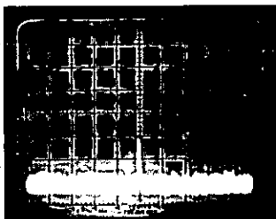
FIGURE 2. The high sensitivity of the 8555A allows the observation of very weak signals such as the distortion product of a microwave mixer as pictured above. The absolute peak amplitude of the signal is -110 dBm. Log reference level (top horizontal line in graticule): -60 dBm. Center frequency: 2.9 GHz.
