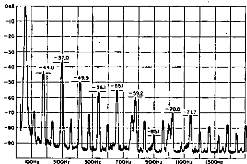
Figure 2. Power line recording using the 3595A
