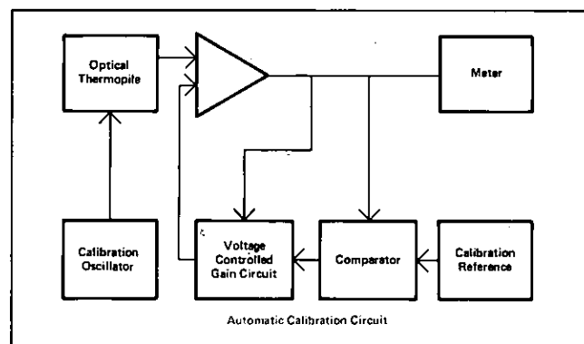
Built-in Calibrator Circuit
