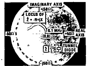
Fig. 2 The complex impedance of active and passive networks may be characterized. Here is the negative resistance characteristic of a tunnel diode from .1 to 10 MHz. Values of -R + jX are easily determined.
