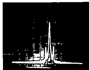
FIGURE 3. The 8555A is capable of resolving low frequency sidebands (1 kHz) which are weak in amplitude (-35 dB) in comparison to the fundamental. Center frequency: 450 MHz. Scan width: 2 kHz/division.
