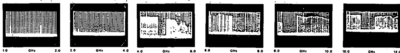
Figure 1. The flat frequency response of the 8555A Microwave Spectrum Analyzer is demonstrated by the series of photos above. Levelled sweep oscillators were used as signal sources over the range from 1 to 12 GHz. The input level was -30 dBm in all bands, and the LOG REF level (top graticule line) is -10 dBm for each photo.
